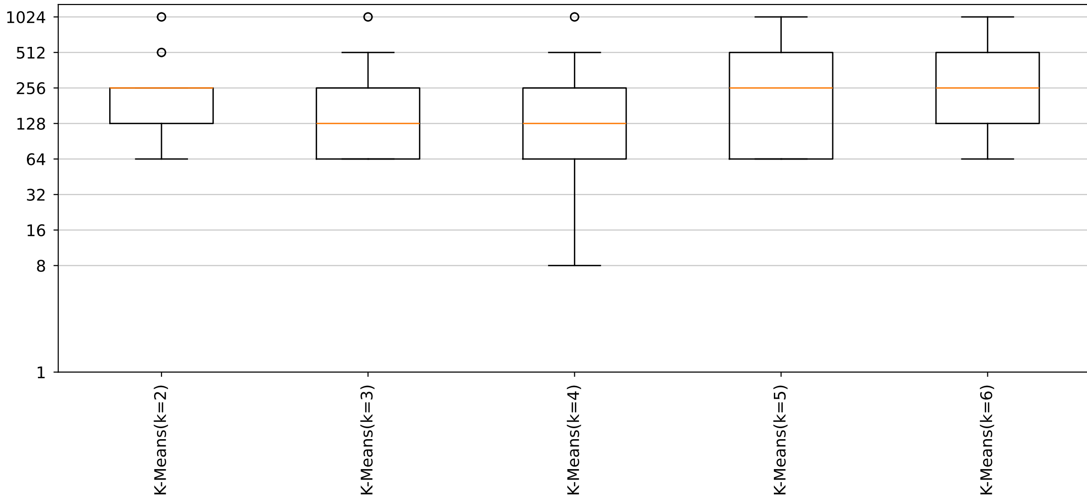
YARA Rules Gram Size Distribution (Cluster18_Size6 dataset)
